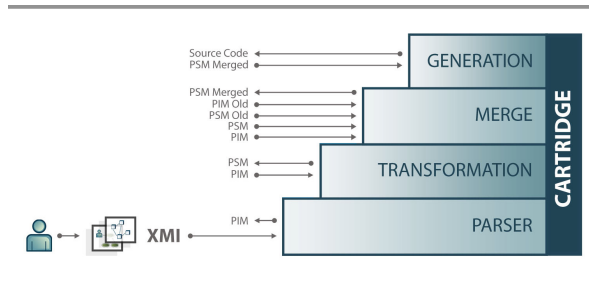
Figure 1: Quantools Architecture
