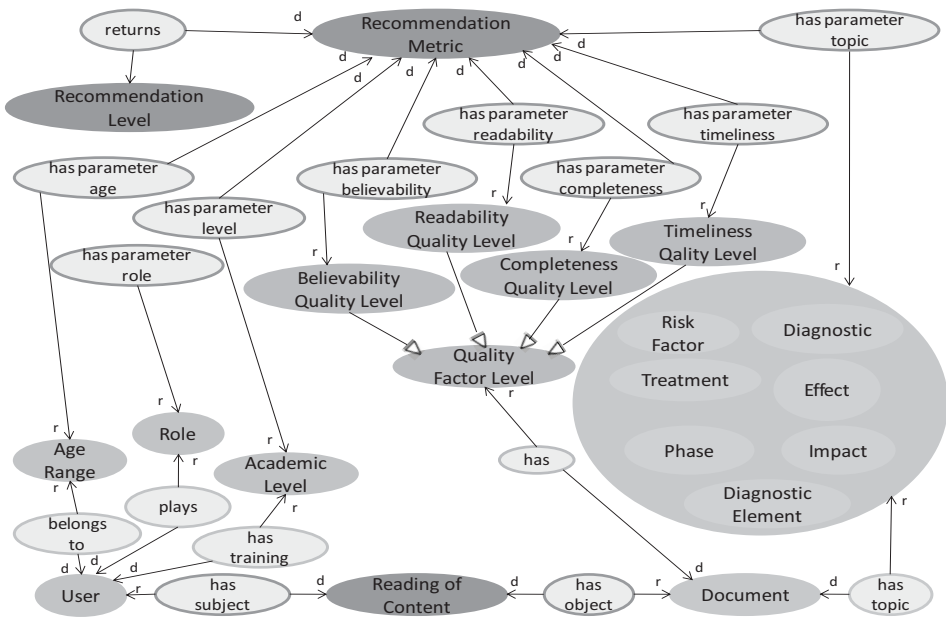
Figure 7. Recommendation Ontology
