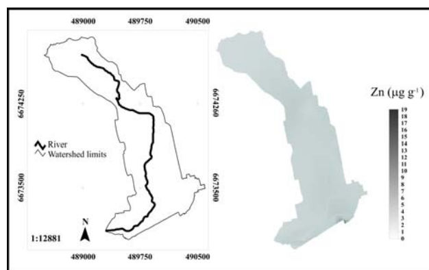
Figure 6 - Distribution of Zn concentrations in urban dusts inside the studied area.
